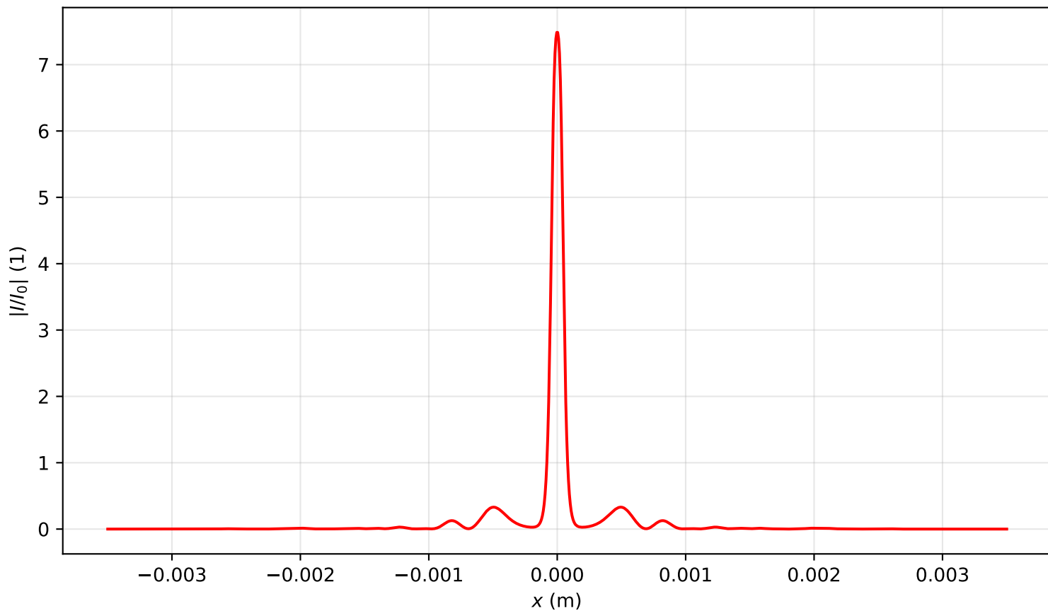
Intensity profile I(x, y = 0, z = 0.478)/I_0 , P_{in}=9.0P_{cr} , artificial time
